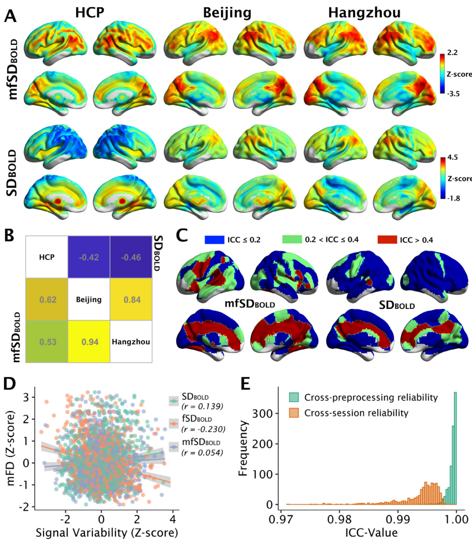
Fig. 1. Reliability and stability of the signal variability measures. (A) Group-averaged spatial patterns of mfSD_{BOLD} (upper panel) and SD_{BOLD} (lower panel) for three datasets. (B) Spatial similarity across sites for SD_{BOLD} (upper triangle) and mfSD_{BOLD} (lower triangle) based on the Fan 246 template. (C) Cross-site reliability of mfSD_{BOLD} (left) and SD_{BOLD} (right) for each brain region. (D) Correlations between signal variability and mFD (each dot represents one participant). (E) Reliability of mfSD_{BOLD} cross two sessions (HCP: REST1 and REST2; orange) and different preprocessing parameters (HCP: with and without global signal regression; green) for each individual participant. SD_{BOLD} , standard deviation of the BOLD signal; fSD_{BOLD} , fractional SD_{BOLD} ; mfSD_{BOLD} , mean-scaled fSD_{BOLD} ; ICC, intraclass correlation coefficient; mFD, mean framewise displacement (For interpretation of the references to color in this figure legend, the reader is referred to the web version of this article.).
